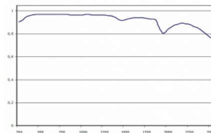
Typical spectral reflection of the sphere coating made of barium sulfate (ODP97).
