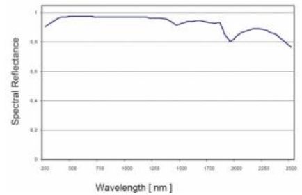
Wavelength [nm] - Typical Spectral Reflectance
