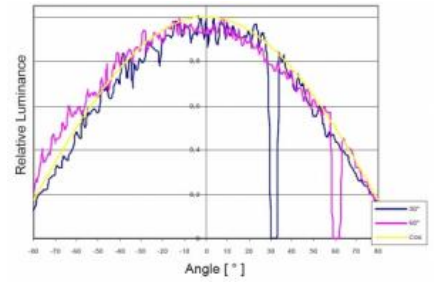
Angle [°] - Typical Diffuse Reflectance Characteristic
